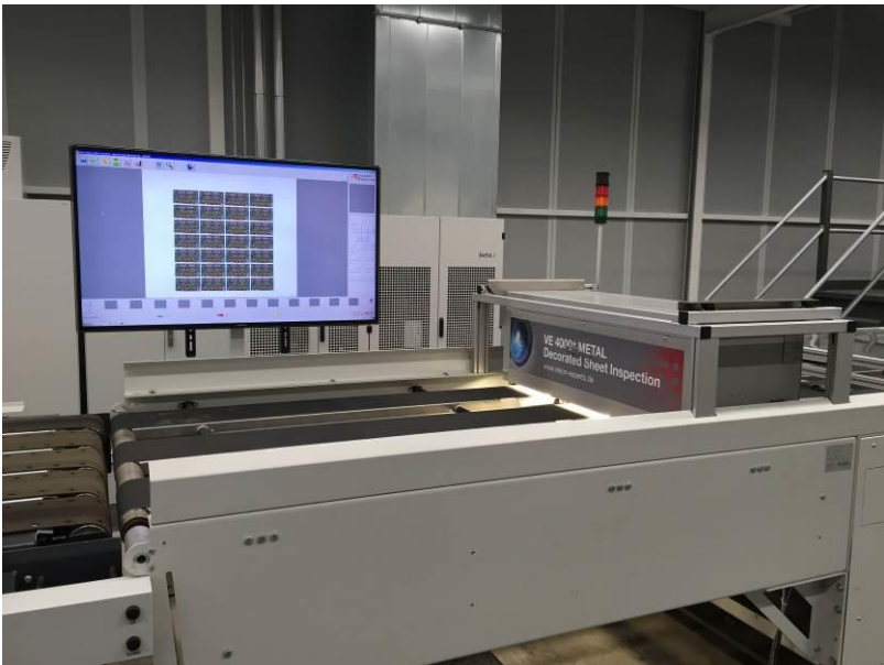
Vision Experts inspection system VE 4000+ Metal
